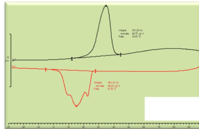
DSC-Analysis: high buffer capacity (50 – 90 J/g)
